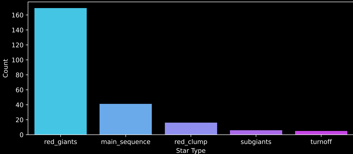
APOGEE DR17 Field: [281+12] Count plot of Star Type
