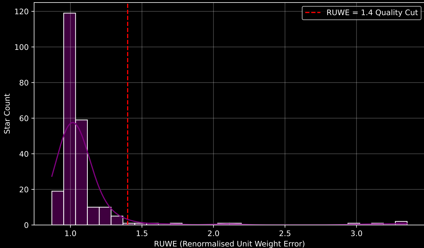
GAPOGEE DR17 Field [281+12] RUWE Distribution (n= 232)
