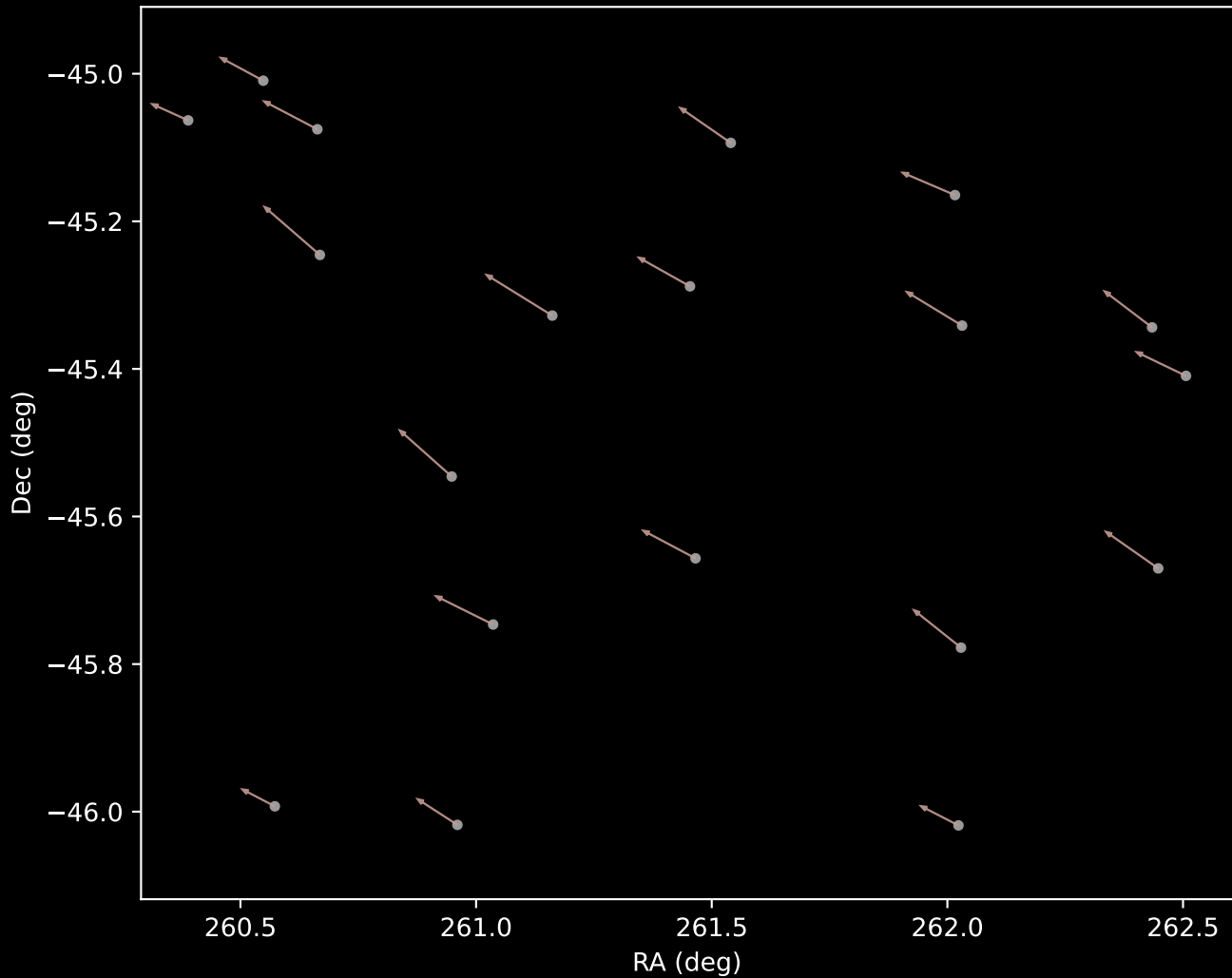
APOGEE DR17 Cluster 11 Proper Motion Vectors (n=19)
